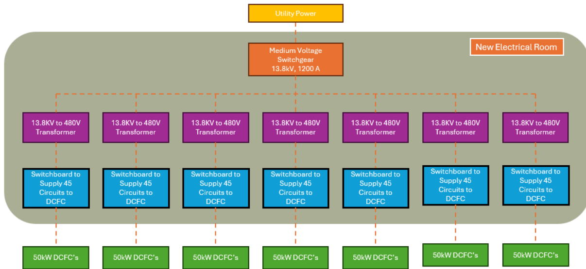
Figure 4 Electrical Layout
