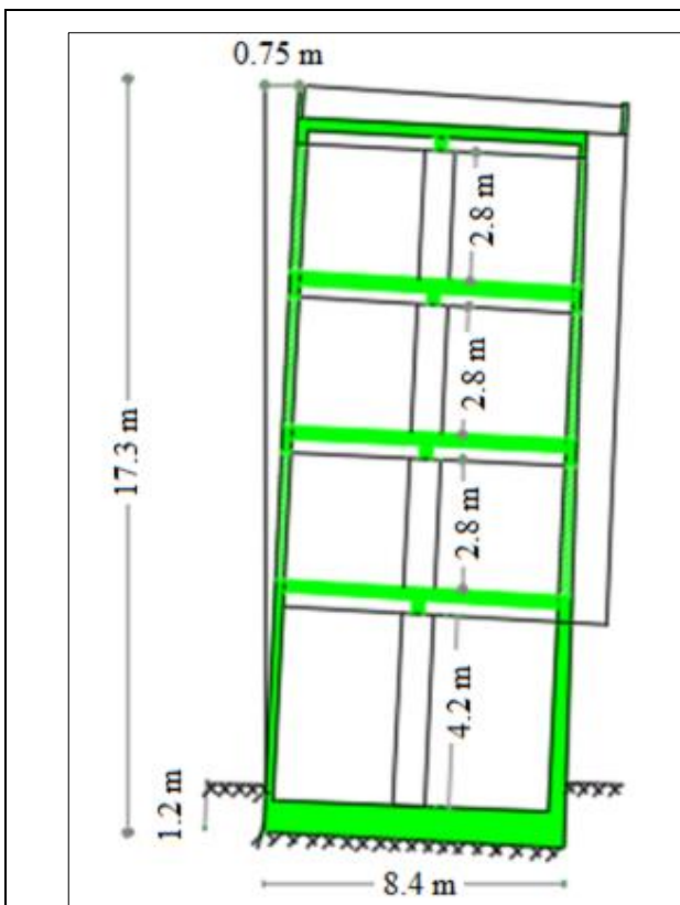
Figure 2 Cross section 1-1 after building tilt
